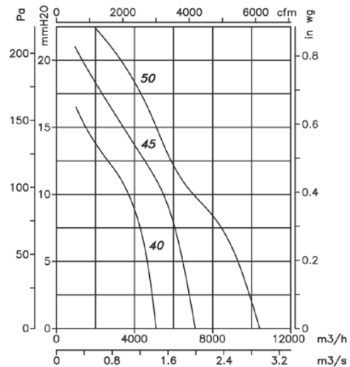
4-Pole=1500 r/min
