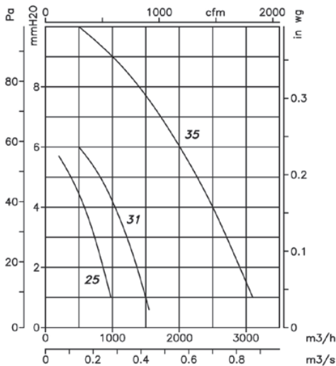
4-Pole=1500 r/min
