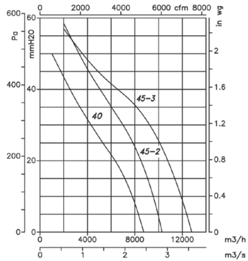
4-Pole=1500 r/min
