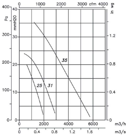
4-Pole=1500 r/min
