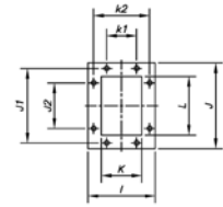
Outlet nozzle 980...1090
